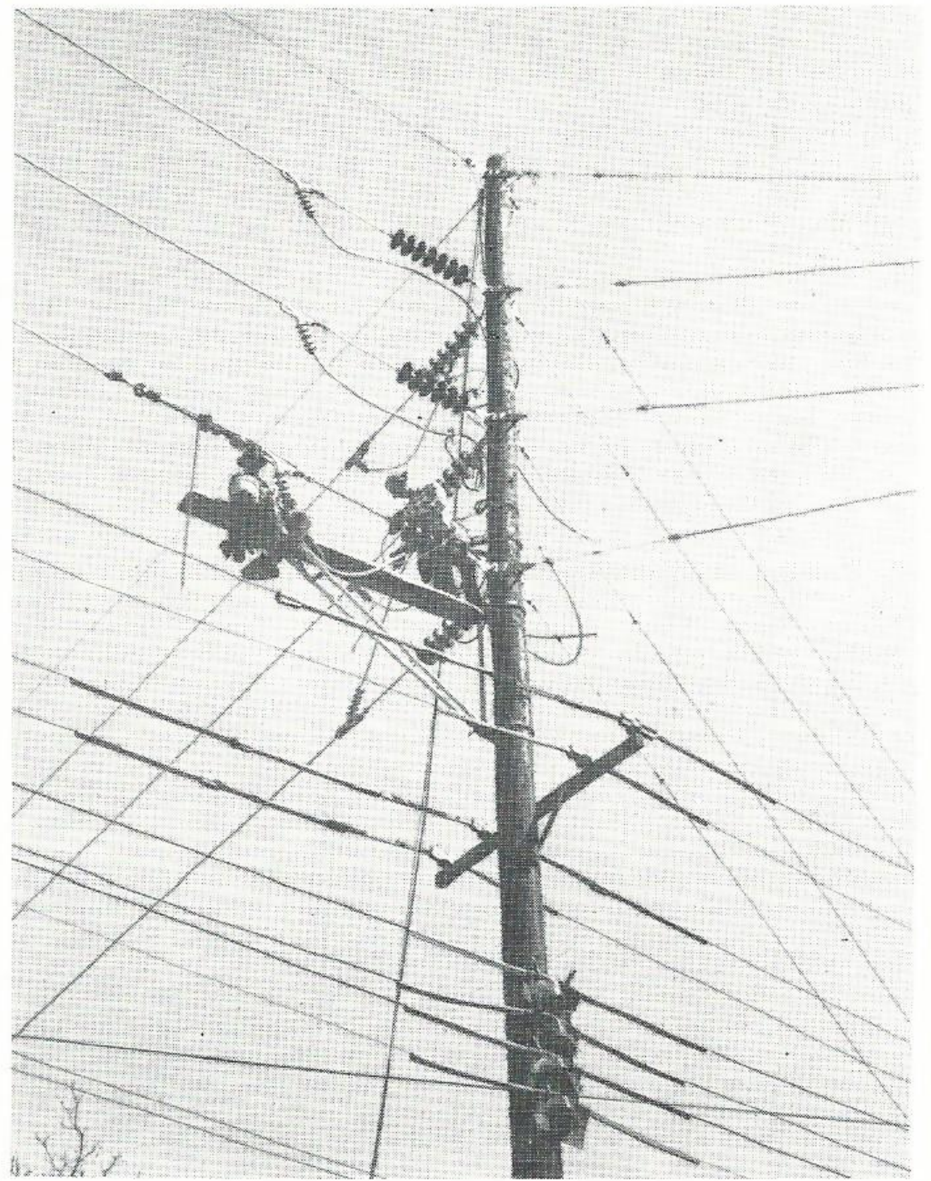
PROGRESS CAUSES WORK, TOO. Harold E. Turner, on pole, and William H. Tholborn, on platform, are sagging 795 aluminum conductors in building a new run-around on 69 Kv line to clear the way for the expressway that is being built through the heart of Baton Rouge. Both men are linemen. Helpers on the hand lines for this job were James W. Bello and Martin J. Munn, Jr., Baton Rouge T&D. Foreman was Joe Mayeux.
