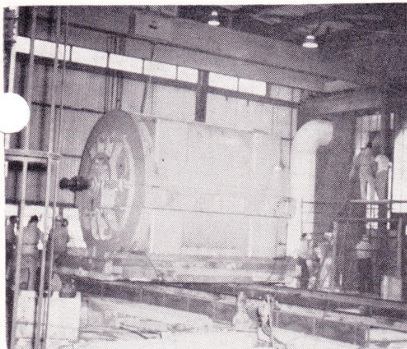
LOUISIANA STATION'S NEW UNIT — a 15,000 kilowatt non-condensing hydrogen cooled turbine generator unit is seen above shortly before it was readied for operation. This addition, numbered Unit 1-A, was placed in commercial operation in October. Being a non-condensing unit, it will be used to furnish part of the steam requirements for the nearby Esso Standard Refinery and Ethyl Corporation.
